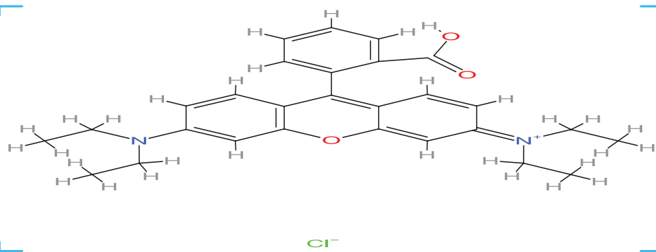
Supplementary Figure 1: Rhodamine B ( \text{C}_{28}\text{H}_{31}\text{N}_2\text{O}_3\text{Cl} ) is an organic chloride salt having N-[9-(ortho-carboxyphenyl)-6-(diethylamino)-3H-xanthen-3-ylidene] diethyl ammonium chloride.
