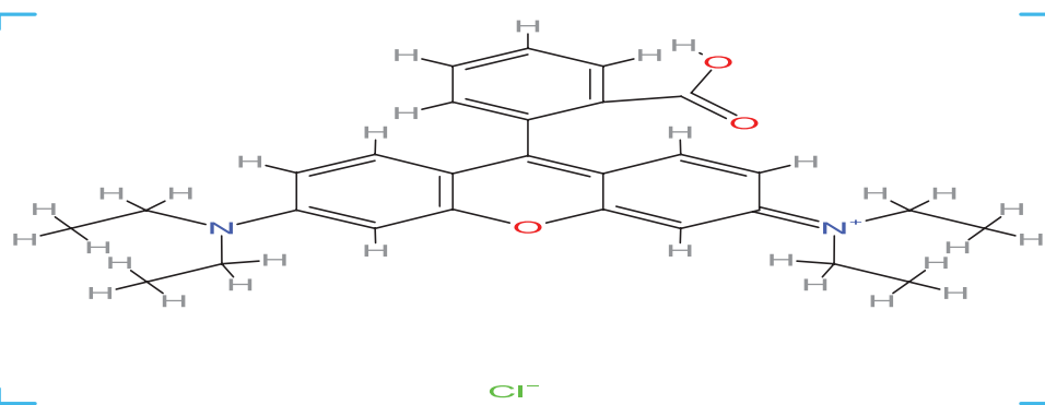
Supplementary Figure 1: Rhodamine B ( C_{28}H_{31}N_2O_3Cl ) is an organic chloride salt having N-[9-(ortho-carboxyphenyl)-6-(diethylamino)-3H-xanthen-3-ylidene] diethyl ammonium chloride.
